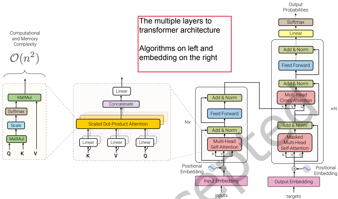
Fig. 1. Architecture of the standard Transformer [82]
